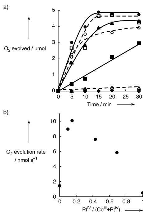
Figure 3. a) Time courses of \text{O}_2 evolution by visible-light irradiation ( \lambda > 420 nm) of a phosphate buffer (2.0 mL, 50 mM, pH 8.0) containing [\text{Ru}(\text{bpy})_3]^{2+} (1.0 mM), \text{Na}_2\text{S}_2\text{O}_8 (5.0 mM), and a heteropolynuclear cyanide complex, [\text{Co}^{\text{II}}(\text{H}_2\text{O})_m]_n[(\text{Co}^{\text{III}}_{1-x}\text{Pt}^{\text{IV}}_x)(\text{CN})_6] (80 \mu\text{g} ). x = 0 (closed square); 0.10 (open square); 0.15 (closed circle); 0.43 (open circle); 0.69 (closed triangle) and 1 (open triangle). Time course of \text{O}_2 evolution under dark conditions using the complex with x = 0.15 (open diamond). b) Initial \text{O}_2 evolution rates (< 5 min) at different \text{Pt}^{\text{IV}} ion contents in [\text{Co}^{\text{II}}(\text{H}_2\text{O})_m]_n[(\text{Co}^{\text{III}}_{1-x}\text{Pt}^{\text{IV}}_x)(\text{CN})_6] .
